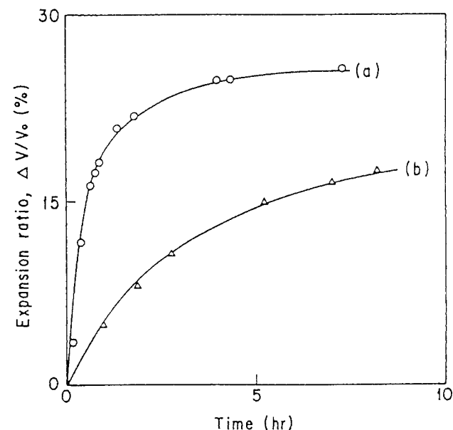
Figure 1. Transient expansion ratios of: (a) NH 4 ClO 4 /ethanol solution; (b) NaSCN/ethanol solution under pressurized carbon dioxide.
